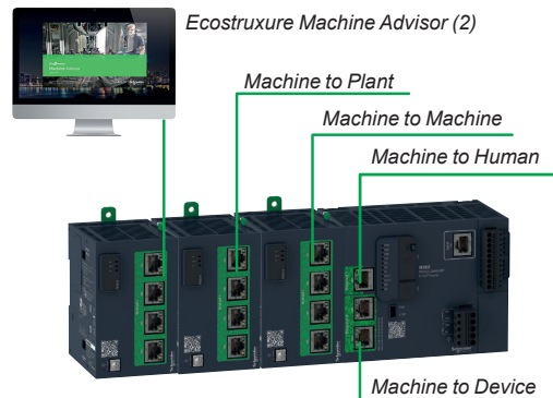
Modicon M262 logic controller with 3x TMSES4 Smart communication modules (maximum configuration)
